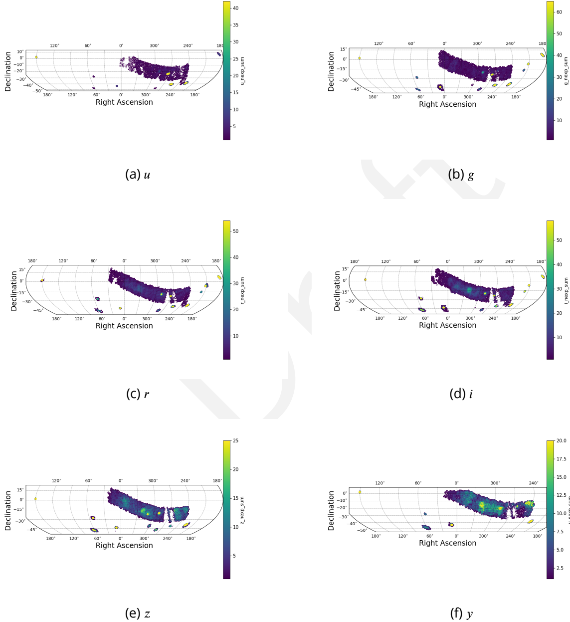
Figure 1: PRELIMINARY EXPECTED DP2 number of input visits to coaddition in each LSST band (ugrizy) based on the QuickLook measurements in ConsDB. Use table 5 to determine the number of visits contributing to deep drilling fields and field surveys taken during First Look.
